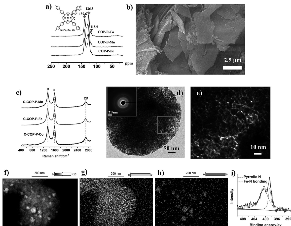
Figure 1. a) Solid-state ^{13}\text{C} NMR spectra of COP-P-M ( \text{M} = \text{Fe} , \text{Co} , and \text{Mn} ); b) SEM image of COP-P-Fe. c) Raman spectra of C-COP-P-M ( \text{M} = \text{Fe} , \text{Co} , or \text{Mn} ); d) TEM image of C-COP-P-Fe. Inset: the selected-area electron diffraction (SAED) pattern. e) An enlarged view of the area within the square in (d). f) TEM image of C-COP-P-Fe for element mapping. g) Carbon atom mapping of the C-COP-P-Fe sample. h) Iron atom mapping of the C-COP-P-Fe sample. i) XPS N 1s spectrum of the C-COP-P-Fe. The N 1s peak can be fitted with two Lorentzian peaks corresponding to Fe–N (398.7 eV) and pyrrolic N (400.6 eV), respectively.
